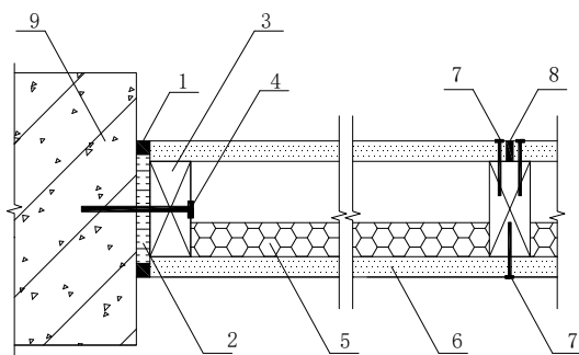
(a) 隔墙
